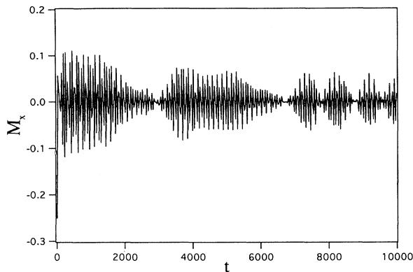
FIG. 19. M_x vs time for the antiferromagnetic HMF. Initially we modulate 50% of the uniform spatial state with wavelength 2\pi . U = -0.4 , N = 10000 . A similar, but approximately out of phase, behavior is observed for the M_y component.
