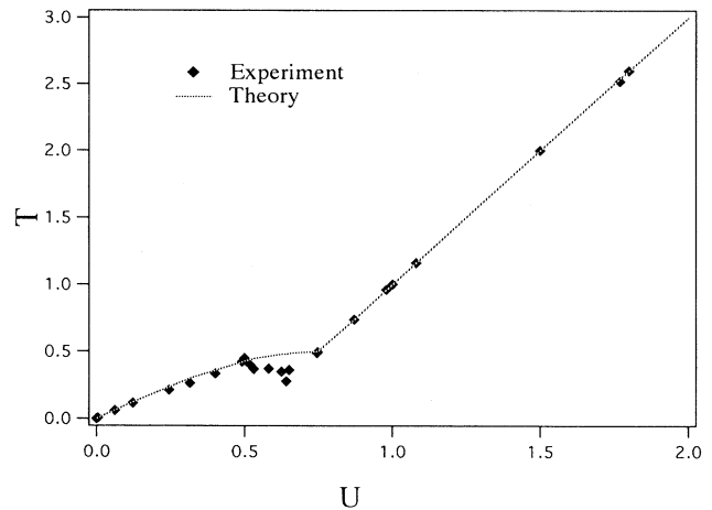
FIG. 4. Temperature (twice the averaged kinetic energy) as a function of the energy U = H/N . The dotted line is the theoretical equilibrium result, the points are results of numerical experiments in the microcanonical ensemble.
