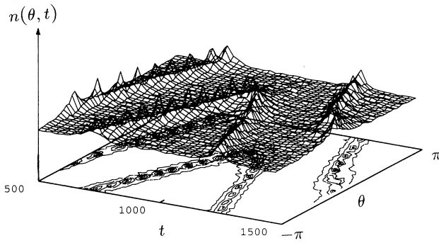
FIG. 7. Plot of the distribution function n(\theta, t) . U = 0.4 , N = 10\,000 . The contour plot is also drawn in the (t, \theta) plane.
