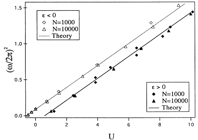
FIG. 15. Dependence of the frequency (\omega/2\pi)^2 given in Eq. (45) on the energy U . The dotted (full) line is the theoretical prediction for \epsilon = -1 ( \epsilon = +1 ) and the points are the values obtained in numerical experiments ( \epsilon = -1 , open symbols; \epsilon = +1 , full symbols). Some of the points correspond to the same value of U and are due to the presence of multiple close frequencies in the spectrum, caused by the relaxation of the initial water-bag distribution.
