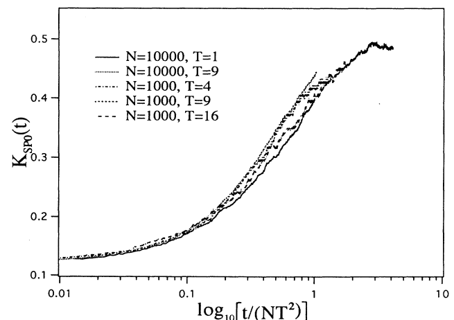
FIG. 14. Temporal evolution of the kinetic energy pertaining to the N/2 low velocity particles in formula (23) with time rescaled by \tau_f = NT^2 with N = 1000 and 10000 and several values of T : T = 1, T = 4, T = 9, T = 16 .
