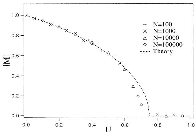
FIG. 3. Modulus of the magnetization in formula (4) as a function of the energy U = H/N . The dashed line is the theoretical equilibrium result, the points are results of numerical experiments performed in the microcanonical ensemble.
