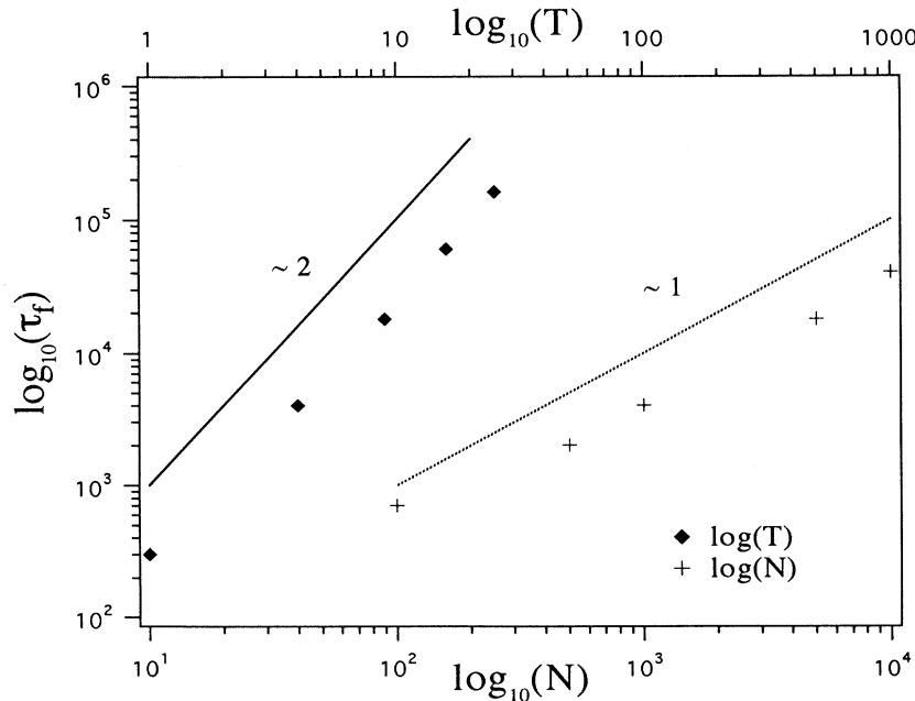
FIG. 12. Relaxation time \tau_f as a function of N with T = 1 (crosses), and vs T with N = 10\,000 (full diamonds). In the figure the theoretical slope 1, corresponding to the N dependence, is also reported (dotted line), together with the slope 2 related to the T dependence (full line).
