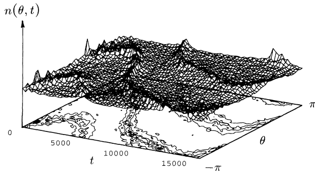
FIG. 16. Plot of the distribution function n(\theta, t) for the antiferromagnetic HMF. U \approx -0.5 , N = 10\,000 . The contour plot is also drawn in the (t, \theta) plane.
