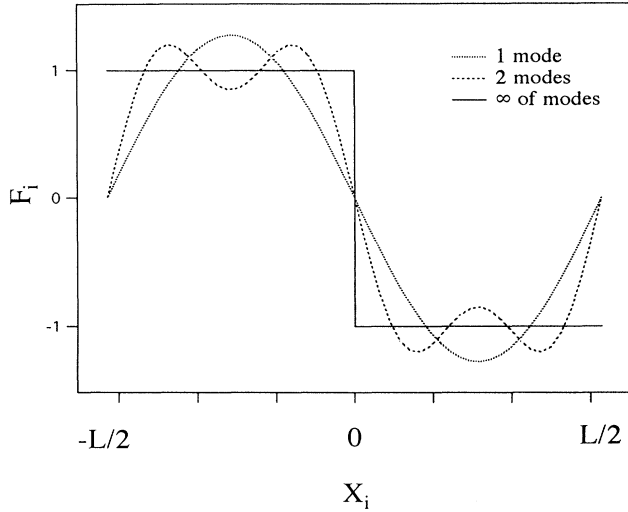
FIG. 2. Behavior of the force F_i in formula (7) with one, two, and an infinity of Fourier components, generated by a particle at position x_i = 0 .
