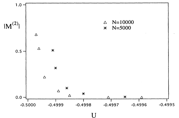
FIG. 18. Modulus of \mathbf{M}^{(2)} in formula (46) as a function of the energy U = H/N , for N = 5000 and N = 10\,000 .
