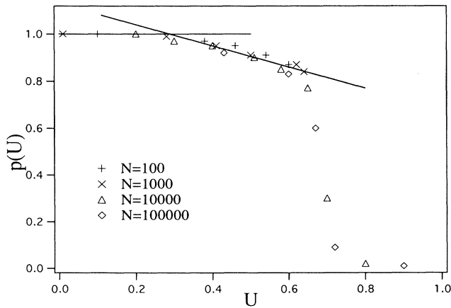
FIG. 5. Trapping probability p(U) as a function of the energy U . The horizontal straight segment is drawn to show that in the bounded subcritical regime p(U) \approx 1 . The other straight segment guides the eyes through decreasing values of p(U) in the translational subcritical regime. The intersection between the two segments determines U_b \approx 0.3 .
