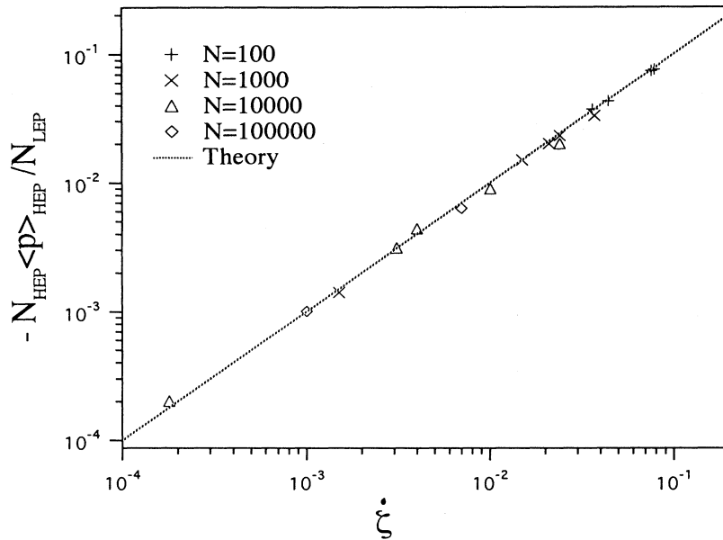
FIG. 9. Relation between the averaged momentum of the high energy particles and the phase drift velocity (22). The dotted line is the theoretical prediction and the points are time averages obtained in numerical experiments. Due to time reversal invariance the same relation holds for negative momentum. The energies vary in the range U_b < U < U_c .
