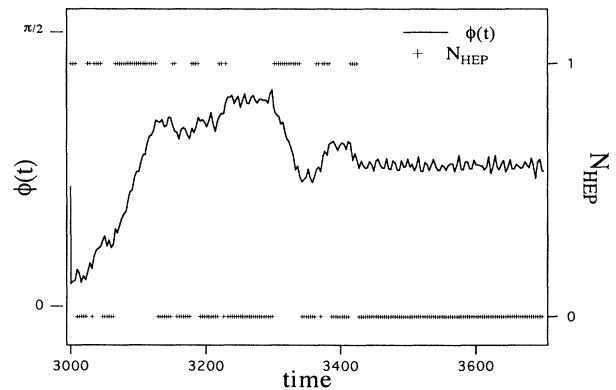
FIG. 6. We plot the phase \phi vs time with a full line. The crosses are set to 1 if there is one untrapped particle, and to zero if all particles are trapped. This shows that phase drift is present only when at least one particle is untrapped. The scale on the left axis is for the phase. N = 100 , U = 0.3 .
