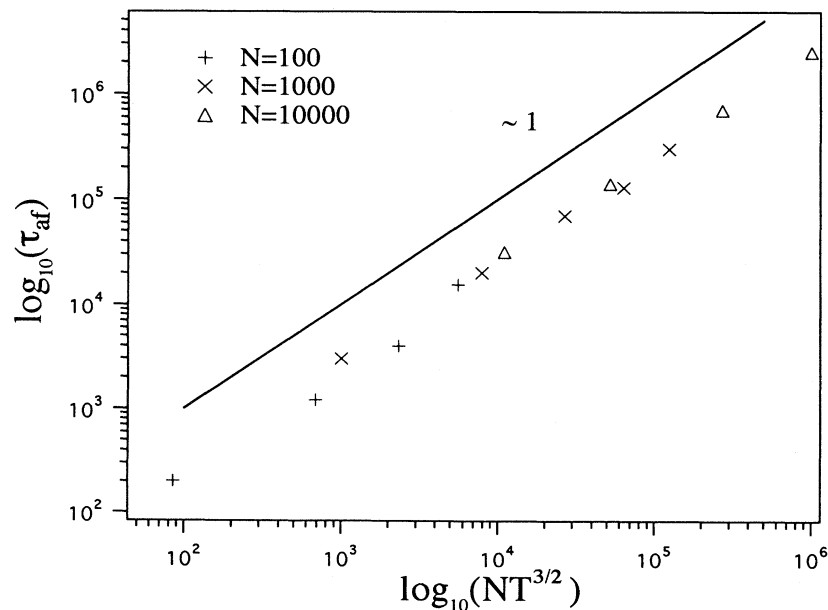
FIG. 20. Relaxation time \tau_{\text{af}} as a function of NT^{3/2} . The points are well fitted by a slope 1.
