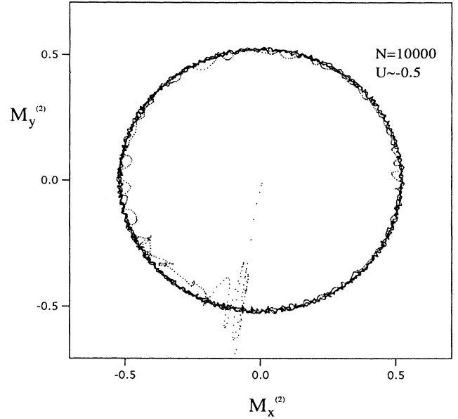
FIG. 17. M_y^{(2)} vs M_x^{(2)} for U \approx -0.5 and N = 10\,000 . The experiment is the same as in Fig. 16. The transient is also shown.
