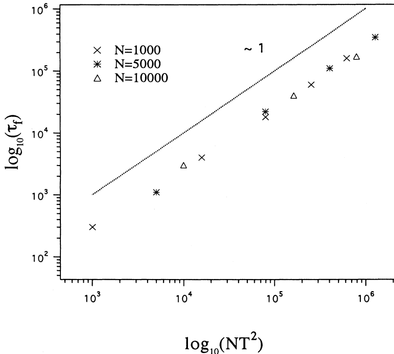
FIG. 13. Relaxation time \tau_f as a function of NT^2 . The points are well fitted by a slope 1.
