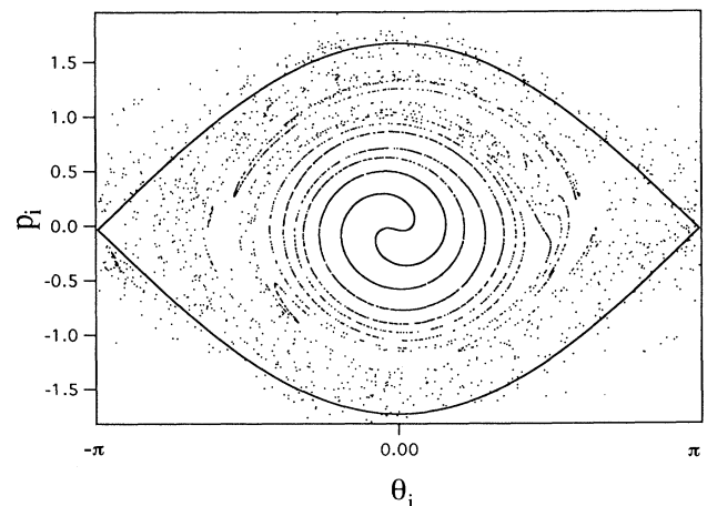
FIG. 11. Boltzmann \mu space for U = 0.4 and N = 10000 in the transient state, together with the separatrix of the perturbed pendulum of Eq. (6) (full line). The experiment is the same as in Fig. 7 and Fig. 8.
