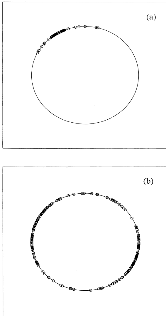
FIG. 1. The particles \pi < \theta_i \leq \pi are all represented by small open circles on the unit circle. (a) Clustering state with U = 0.05 , N = 1000 , \epsilon = 1 . (b) Two-cluster state with U = -0.499 , N = 1000 , \epsilon = -1 , very close to the ground state.
