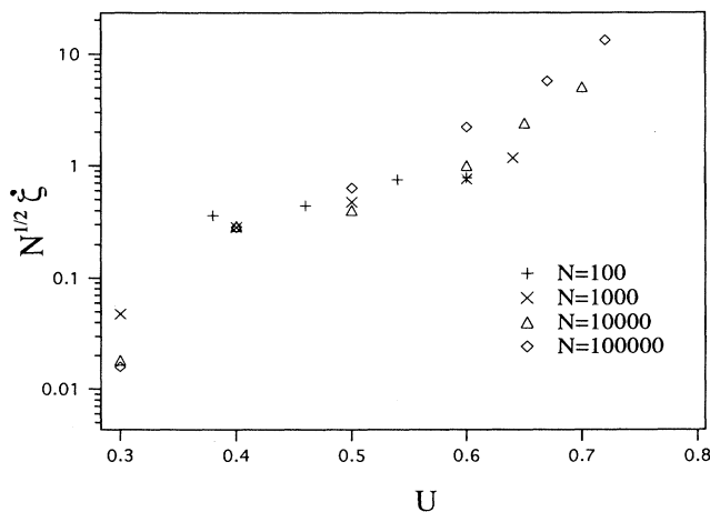
FIG. 10. N^{1/2} \dot{\zeta} as a function of U . The data collapse prove the scaling of \dot{\zeta} as N^{-1/2} for various values of U .
