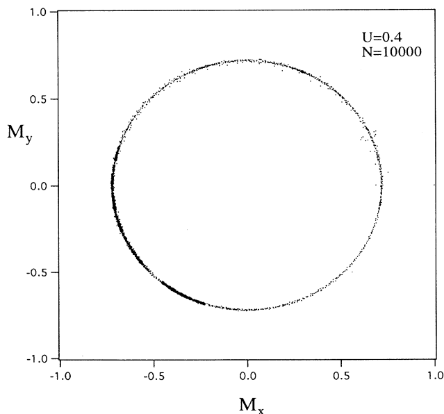
FIG. 8. M_y vs M_x for U = 0.4 and N = 10\,000 after a transient. The experiment is the same as in Fig. 7.
